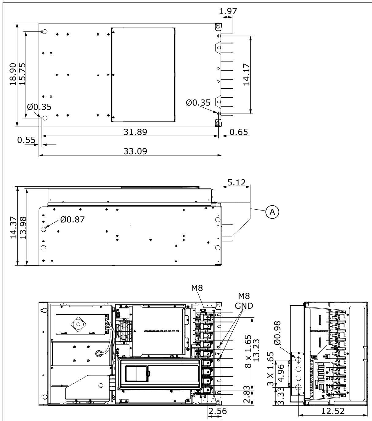
Fig. 17: The dimensions of the AC drive, MR9, UL Open Type [in]
