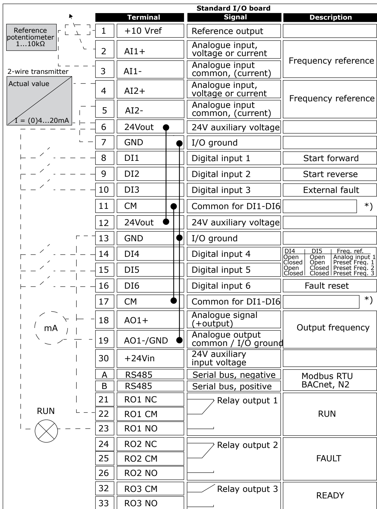
Fig. 39: The signals of the control terminals on the standard I/O board, and a connection example. If you include the optional code +SBF4 in your order, the relay output 3 is replaced with a thermistor input.
