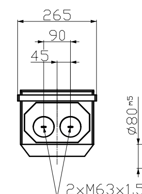
Terminal box - Front view
