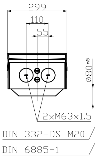
Terminal box - Front view
