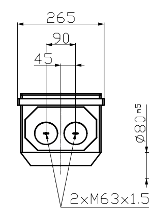
Terminal box - Front view
