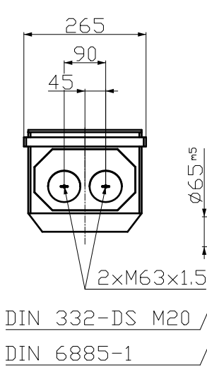
Terminal box - Front view
